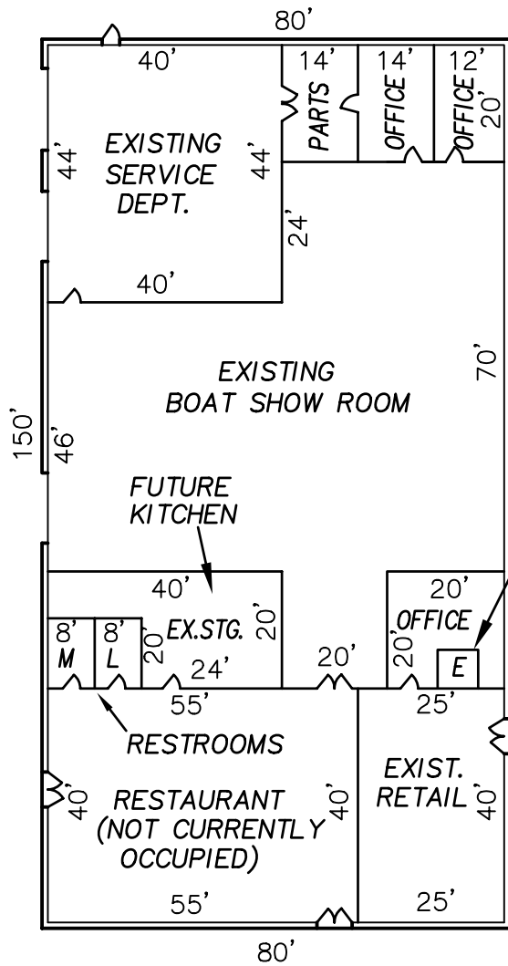
FIRST FLOOR
